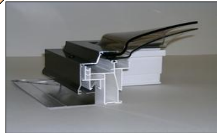
Cross Section of MSF acrylic dome
